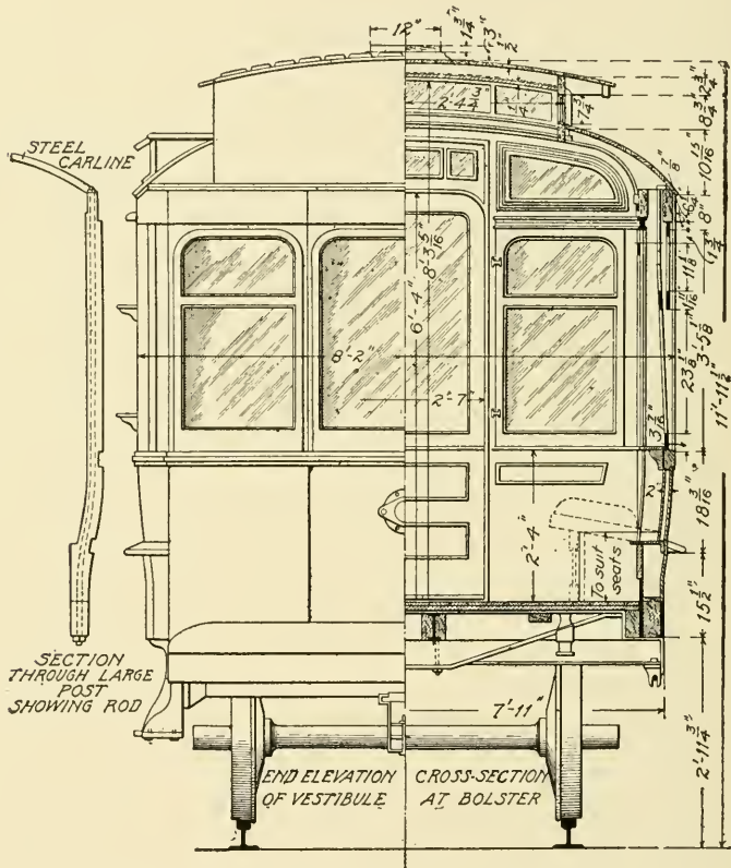
Fig. 3. End View and Cross-Section of Interurban Car
